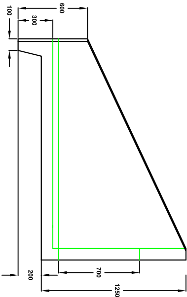
Detail 'B'
