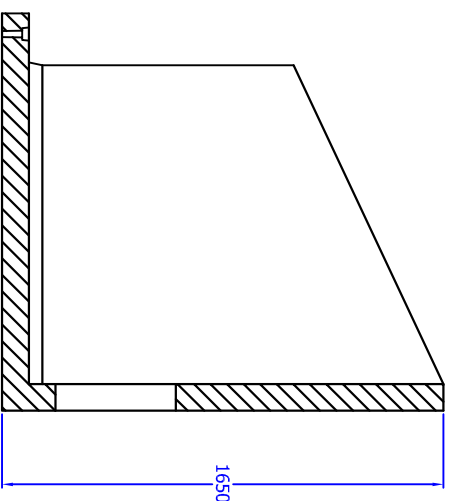
Section XX
