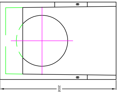
Front elevation with grating removed.
