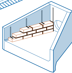
DOVETAIL SLOTS CAST IN TO ALLOW CLADDING OF WINGWALLS AND BACKWALL
